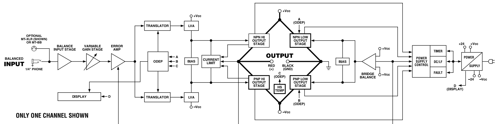
Figure 6.1 Circuit Block Diagram
