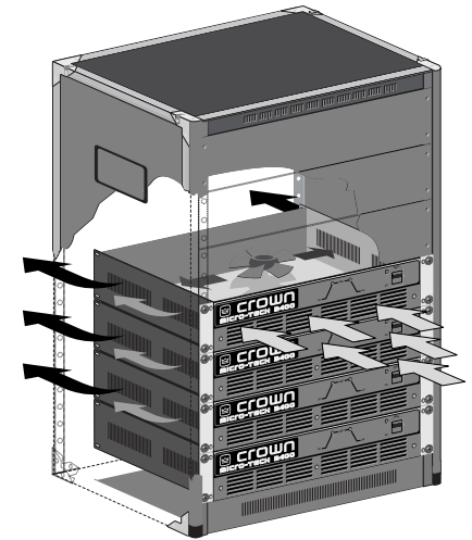
Figure 3.2 Airflow
