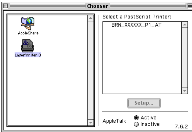
Figure 2 Macintosh Chooser
